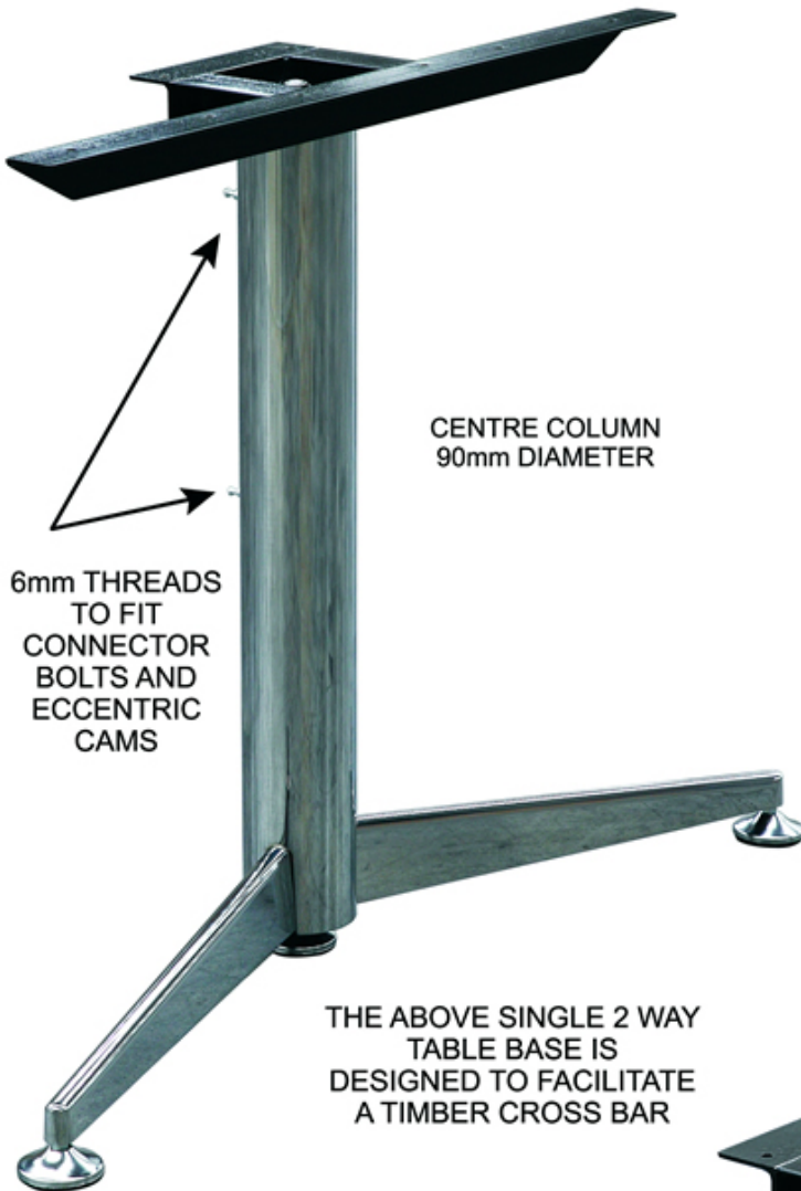
STRAIGHT LEG 2 WAY x 970mm
