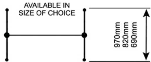
STRAIGHT LEG CONFIGURATION 2 WAY TWIN END (TE SC)
